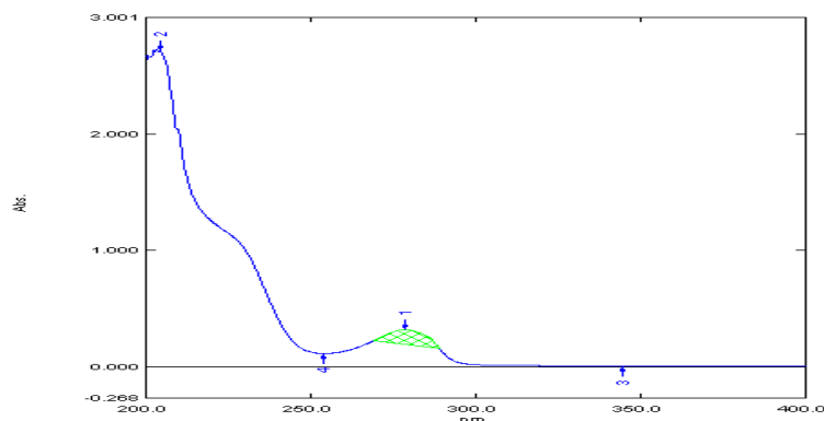
Fig. 5: Area under curve ultra violet -spectra of Aliskiren
