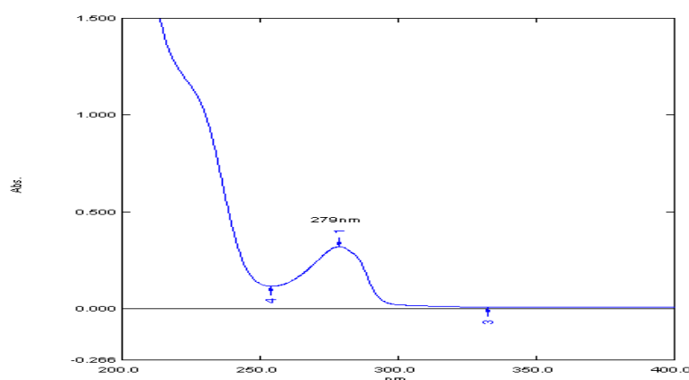
Fig. 2: Zero order UV-spectra showing \lambda_{\text{max}} of Aliskiren
