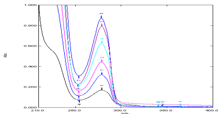
Fig. 3: Overlay spectra representing different concentrations of Aliskiren
