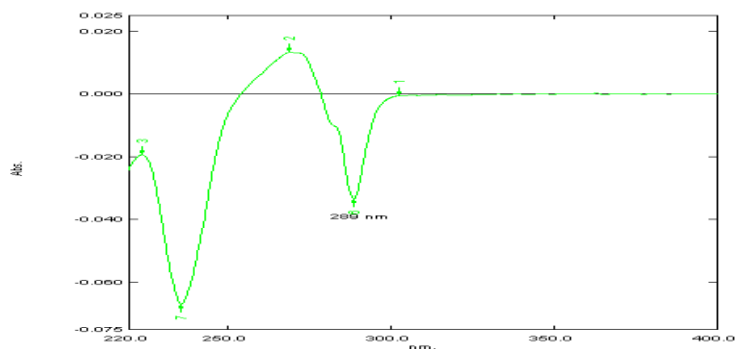
Fig. 4: First order derivative ultra violet-spectra of Aliskiren
