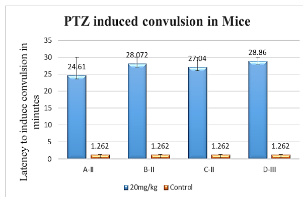
Fig. 3: Graphical representation of Latency to induce convulsions of some synthesized derivatives of N-(5-(Substituted)-1,3,4-thiadiazol-2-yl)-2-((5-(substituted)-4H-1,2,4-triazol-3-yl)amino)acetamide in mice using PTZ induced convulsions
