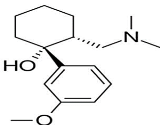
Fig. 2: Tramadol
