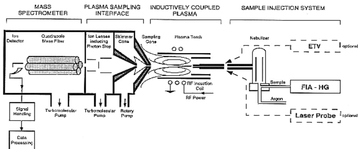
Fig. 1: A: Diagram of inductively coupled plasma mass spectrometry
