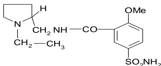
Fig. 1: Chemical structure of Levosulpiride
