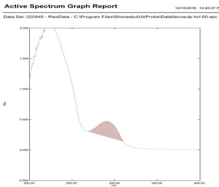
Fig. 2: Area under Curve Spectrum of Levosulpiride in 0.1 N HCl
