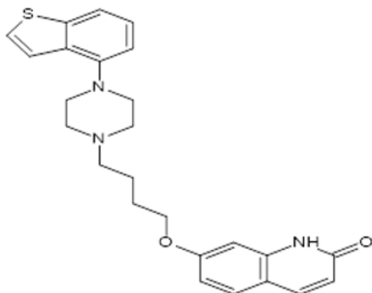
Figure 1: Structure of Brexpiprazole 8
