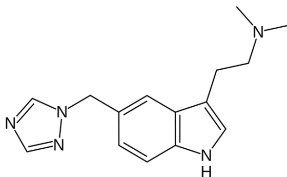
Fig. 1: Chemical structure of Rizatriptan Benzoate
