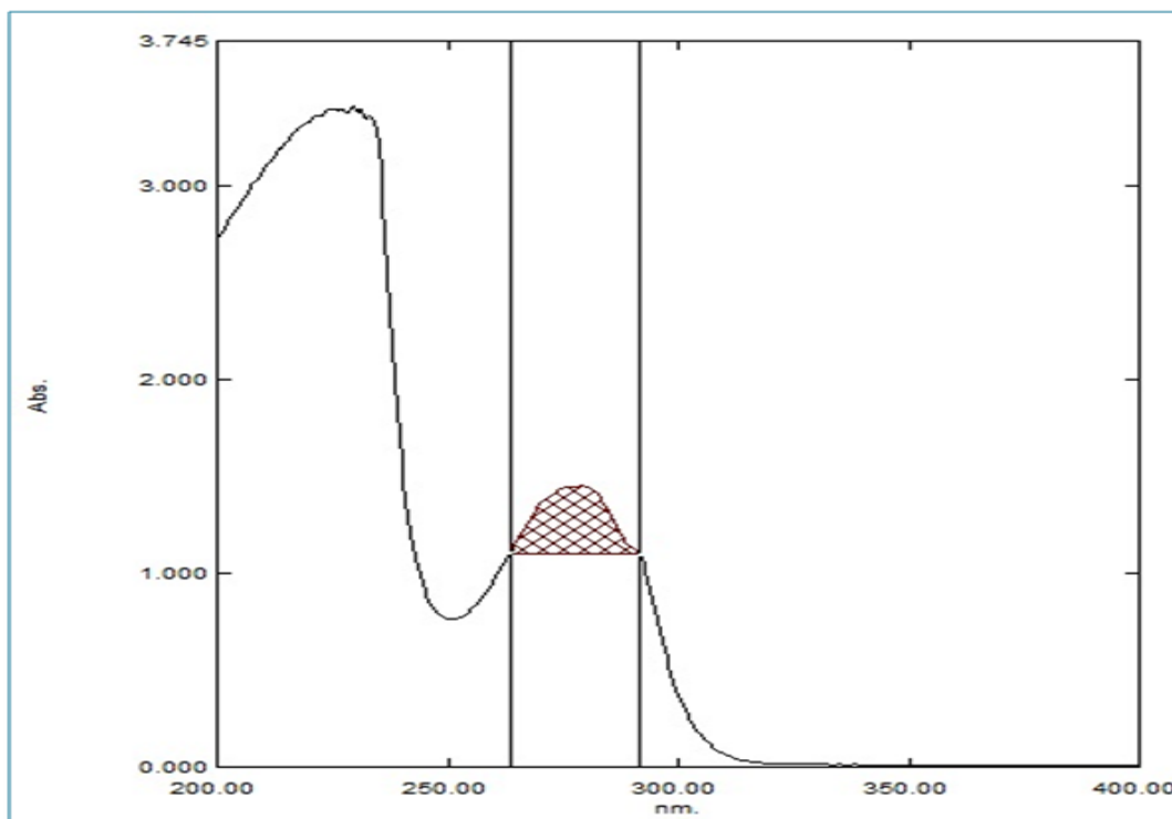
Fig. 2: Area under curve spectrum of Rizatriptan Benzoate in water
