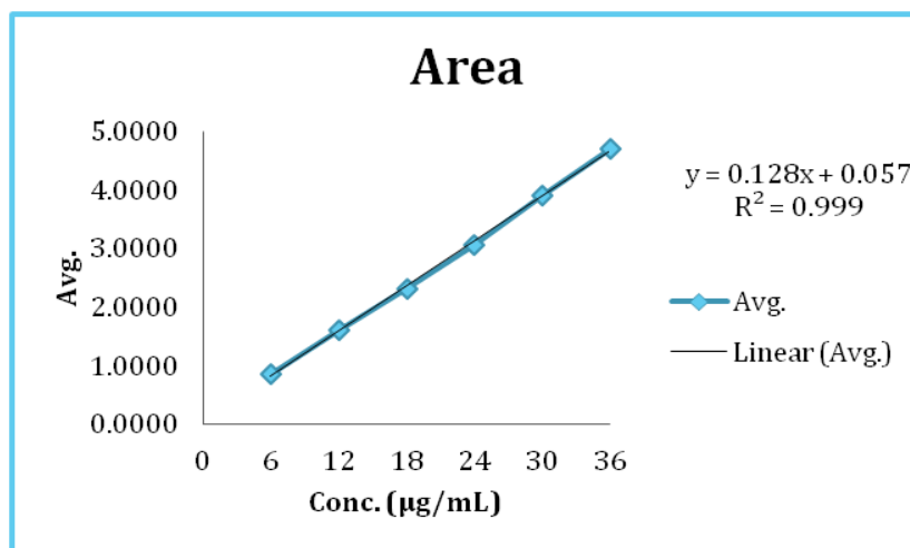
Fig. 3 Calibration curve of Rizatriptan Benzoate
