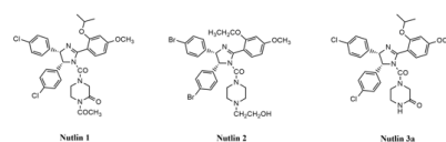
Fig. 6: Structures of nutlins
