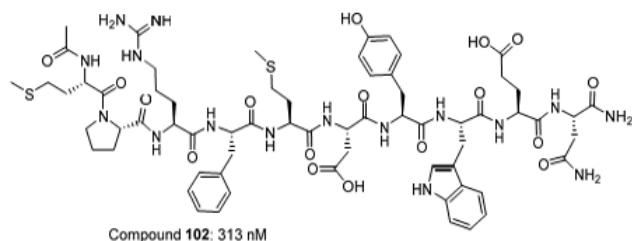
Fig. 5: Structure of peptide inhibitor reported by Novartis
