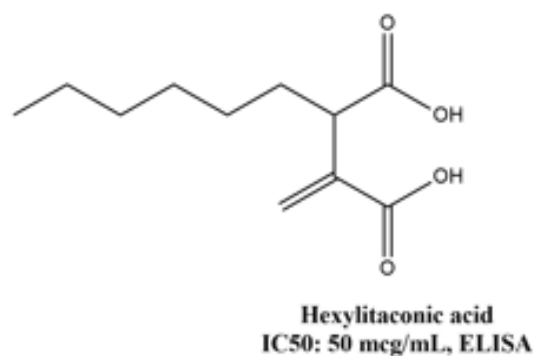
Fig. 4: Structure of hexylitaconic acid
