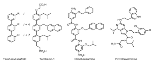
Fig. 7: Structures of \alpha -helix mimetics inhibitors 15
